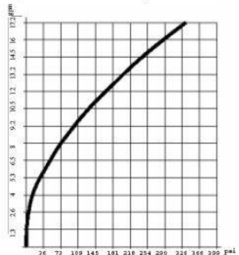
FLOW CHART vs PRESSURE (STRAIGHT NOZZLE)
